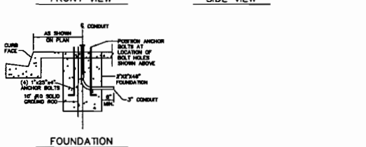
DETAIL "E" NOT TO SCALE
